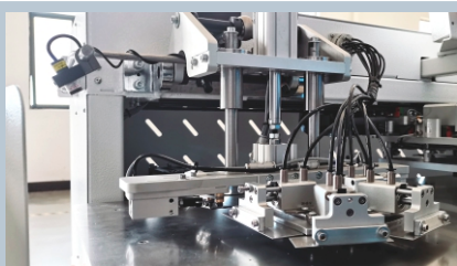
激光对位及自动折叠装置 Laser alignment and automatic folding device
