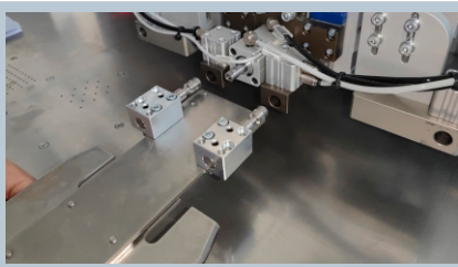
1分钟快速气锁换模 Pneumatic lock jig changing in 1 minute
