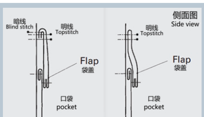
可缝制多种袋盖 For multiple pocket flap styles 明线袋盖口袋 pocket with topstitch flap 暗线袋盖口袋 pocket with blind stitch flap
