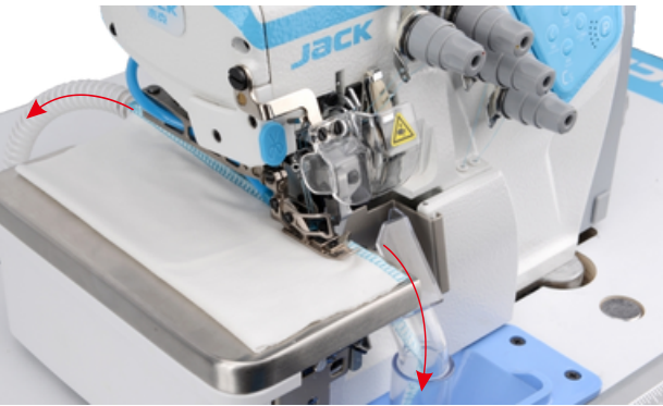
1 Front and Back suction. Clean sewing The front suction for rags ,The back suction for thread tail ,Keep clean sewing
