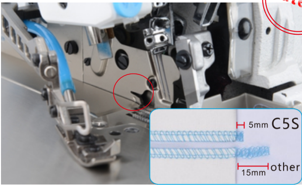
2 Short thread remaining, No need extra trimming Suction trimming, Can control the remaining thread to be within 5MM, No need extra trimming
